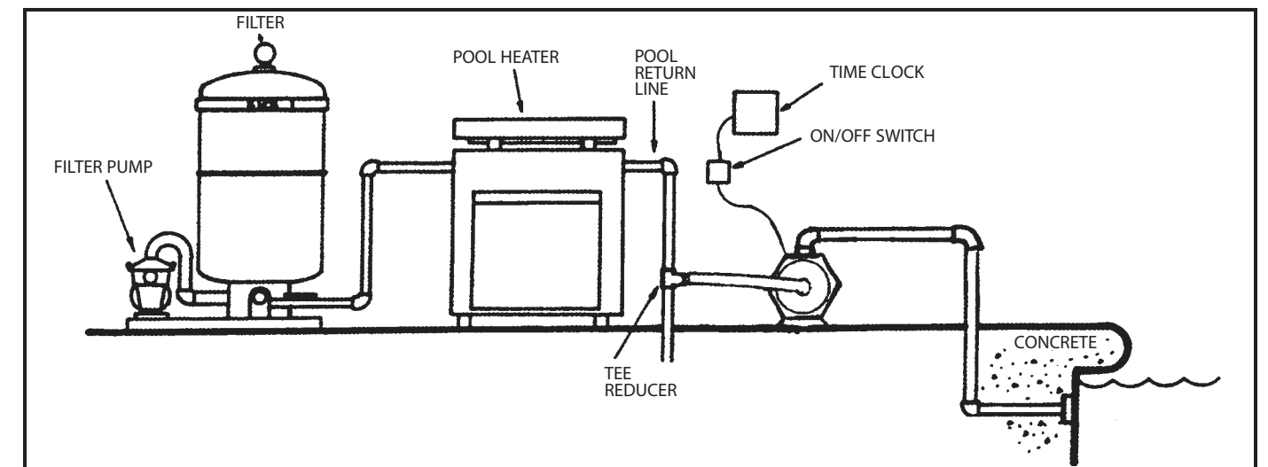
Figure 1: Typical Installation
