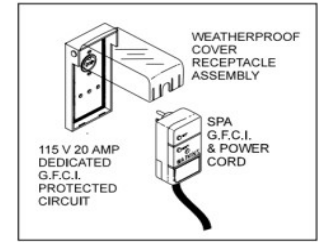
20a Cord, Plug, Outlet
